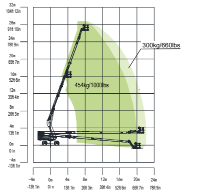
Range of Motion ZT26J
