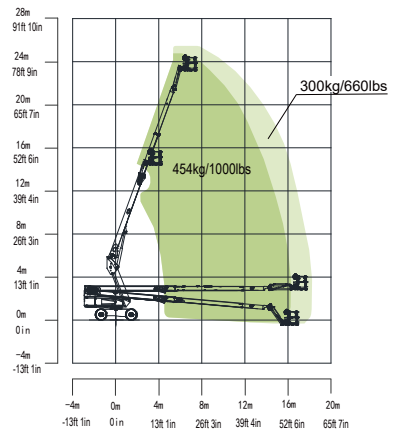
Range of Motion ZT23J
